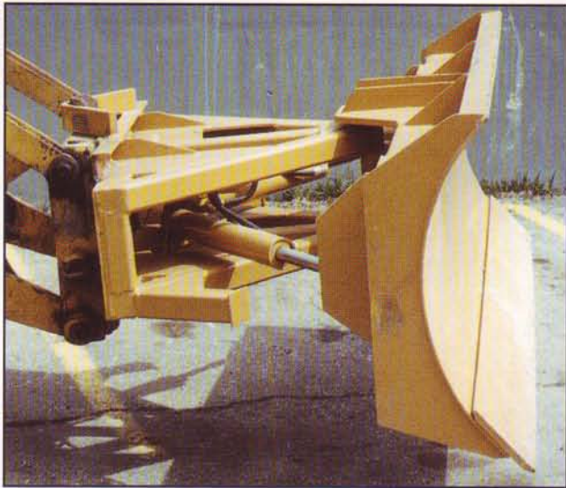
SRD ANGLE DOZER BLADE AND PLOW
